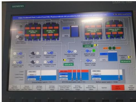
SCADA Project @ DBL Pharma
