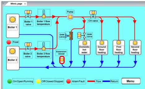
Hot Water SCADA Project
