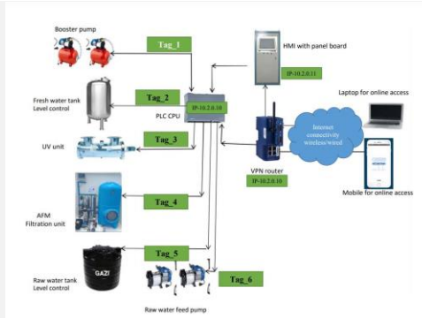
Industrial IIOT Project
